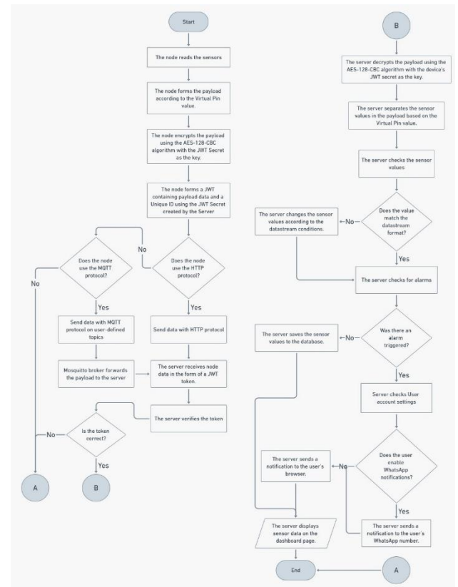
Fig. 5. IoT Device Flow Chart
